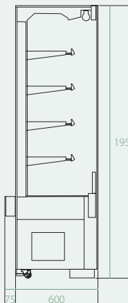
SECTION ELEVATION
