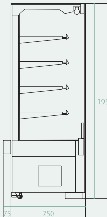
SECTION ELEVATION
