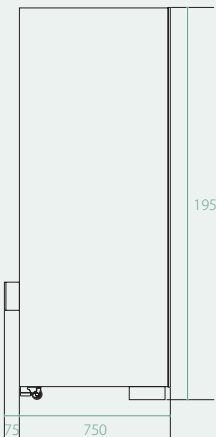
SIDE ELEVATION
